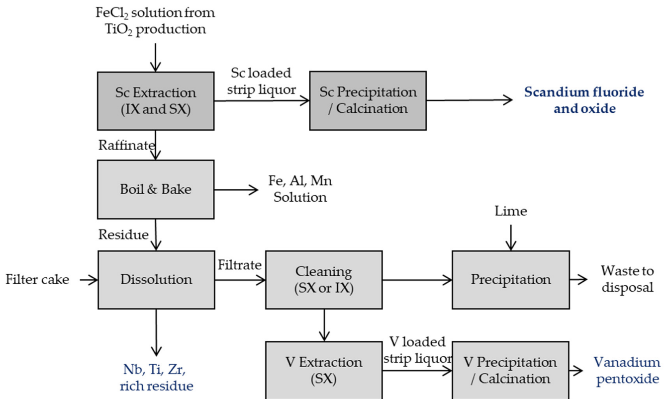
Figure 1. Conceptual process flow sheet of ScaVanger.
