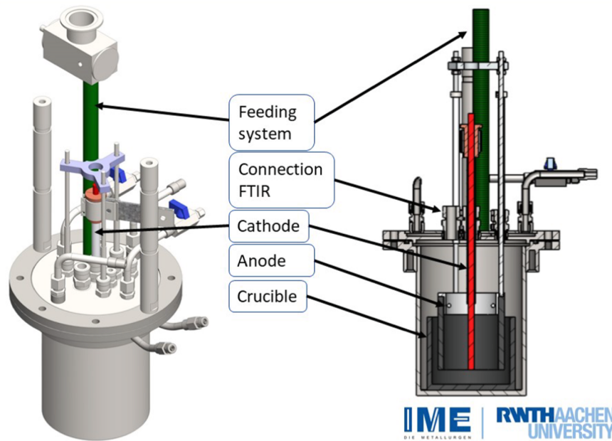
Fig. 1. The experimental setup of the Molten Salt Electrolysis includes a feeding system, Connection FTIR, Cathode, Anode, and Crucible.
