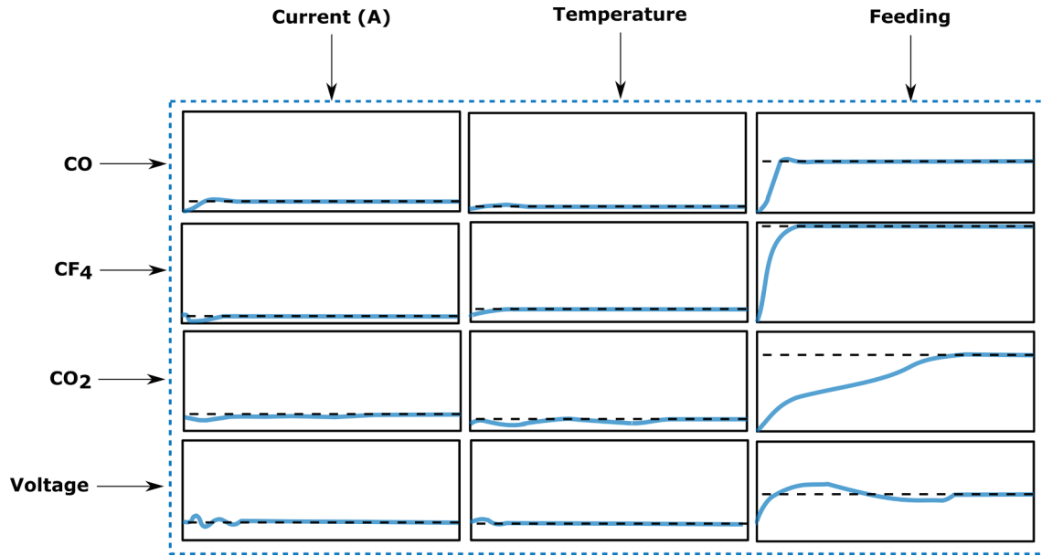
Fig. 4. The step response of the outputs (CO, CF 4 , CO 2 , and Voltage) related to inputs (Current, Temperature, and Feeding).
