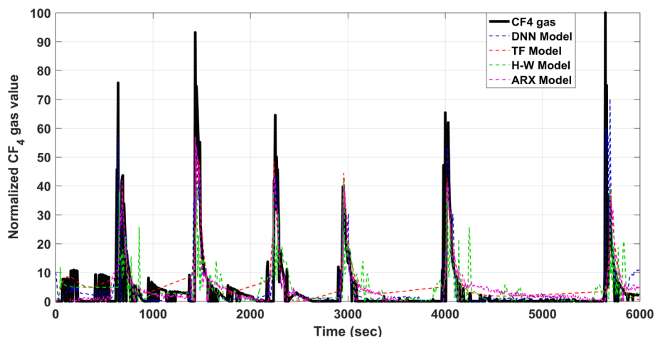
Fig. 10. measured and modelled \text{CF}_4 gas emissions as one of the outputs of the Molten Salt Electrolysis.
