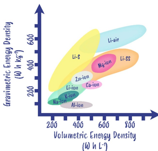
Figure 30. Next generation battery technologies being investigated, and their estimated power and energy densities.
