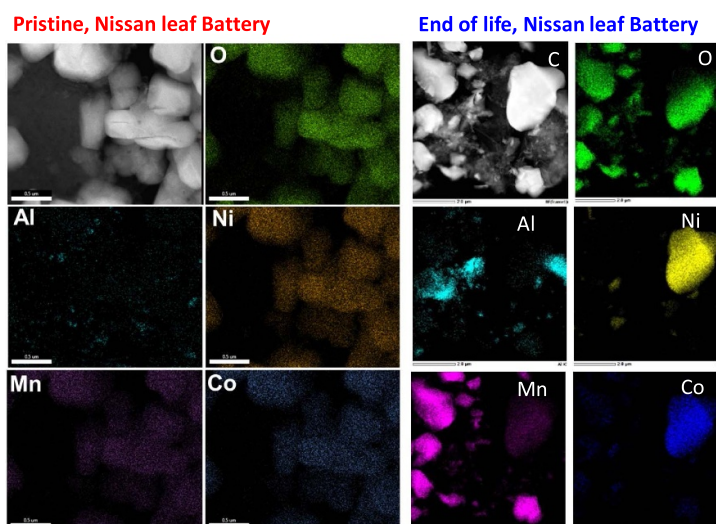
Figure 12. STEM-EDX maps showing the presence and distribution of Al in (a) a pristine and (b) an end-of-life cathode from a first generation Nissan leaf battery. Over the extended cycling of the battery, Al containing phases appear to increase and form primarily at grain boundary triple pockets. Large Al phases has an effect on degradation, recycling and second life applications of LIBs. Reproduced from [148]. CC BY 4.0.
