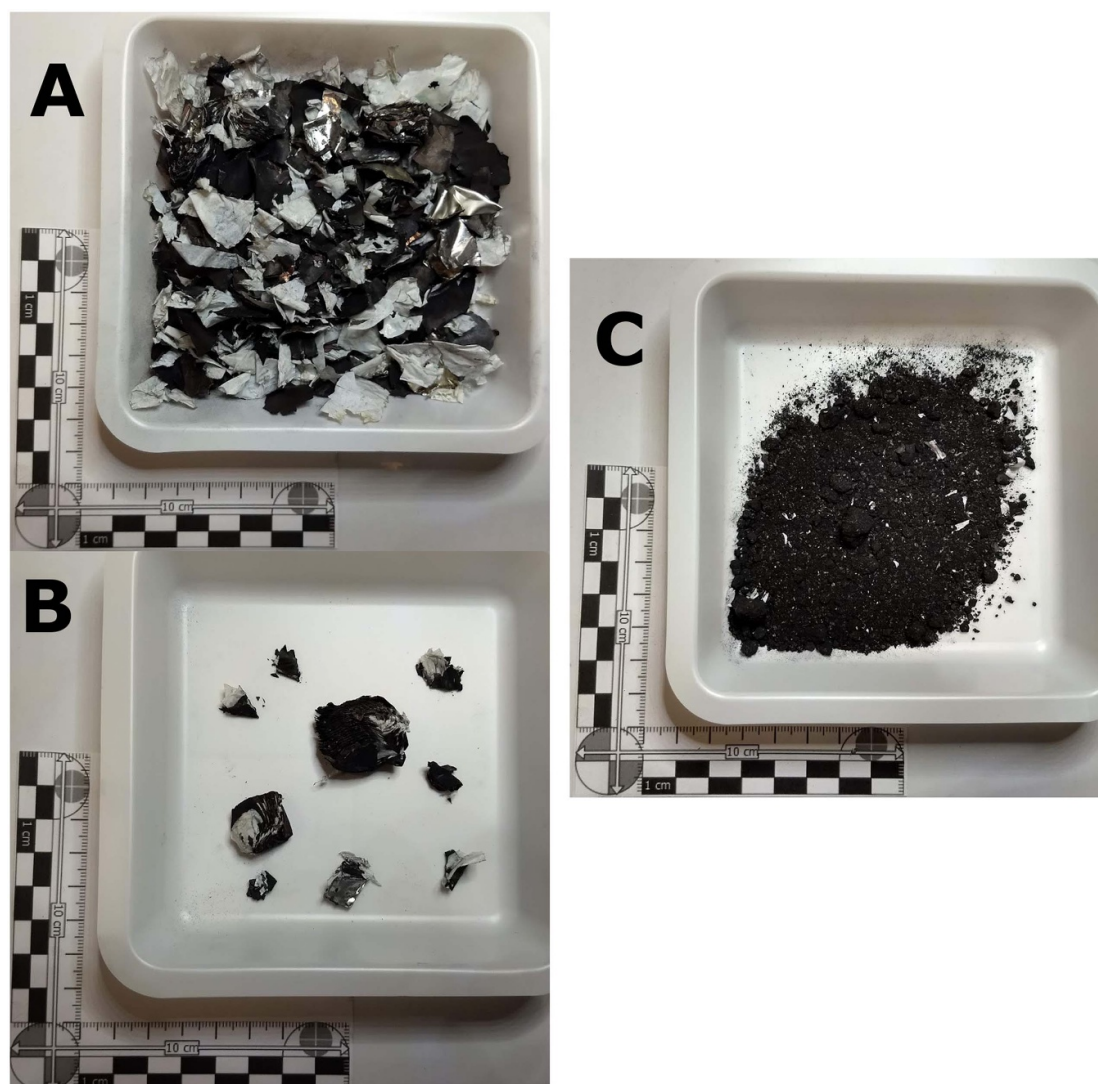
Figure 7. Coarsely shredded material (a). Unliberated material from coarse fraction with inclusions (b). Black mass contaminated with Cu, Al and plastics (c).
