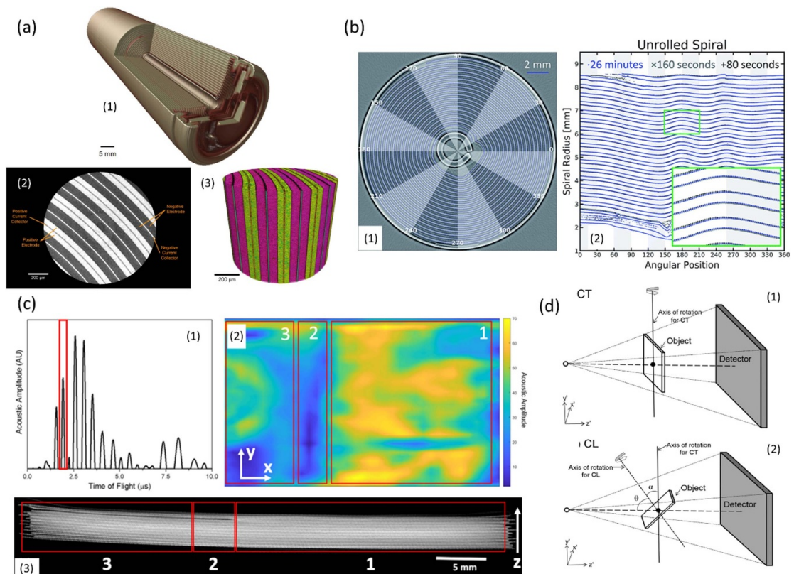
Figure 2. (a) x-ray CT of 18 650 battery: (a1) 3D image of the entire 18 650 cell reveals the spiral cell architecture, inner mandrel, and cell safety devices; (a2) an enlarged region from (a1) examines finer layer details; (a3) the virtual slices were rendered in a 3D volume. Reprinted from [71], Copyright (2017), with permission from Elsevier. (b) Virtual unrolling of 18 650 Li-ion cells: (b1) slice of a cell after edge enhancement (the blue line shows the contour); (b2) A plot of the radius of the spiral versus the angular position for three different acquisition times. Reproduced from [72]. CC BY 3.0. (c) Diagnostic analysis of a Li-ion pouch cell with a defect using correlative methods: (c1) a sample acoustic signal from the area without the defect highlighting the third layer within the cell as the peak of interest; (c2) a 2D raster of acoustic scans corresponding to the amplitude variations of the peak at ca. 2.0 \mu\text{s} (with a 0.4 \mu\text{s} range applied to account for small ToF shifts); (c3) 2D slice of the reconstructed cell confirming the defective region. Reproduced from [73]. © The Author(s). Published by IOP Publishing Ltd CC BY 4.0. (d) Schematic diagrams showing (d1) a conventional circular scan computed tomography (CT) setup, and (d2) the computed laminography (CL) setup. Reproduced from [70]. © IOP Publishing Ltd CC BY 3.0.
