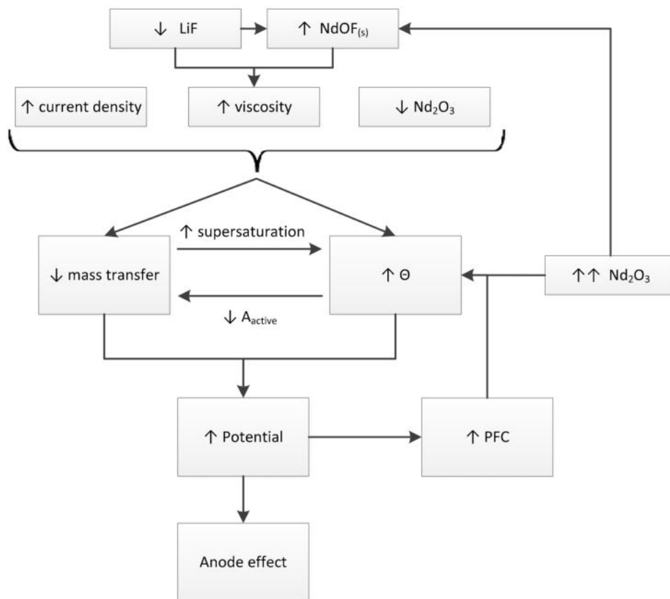
Figure 8. Schematic representation of the relation of the overall cell potential to different factors considered in this study. Arrows in the block: ↑ —increase; ↓ —decrease; ↑↑ —high feeding rate or above saturation.
